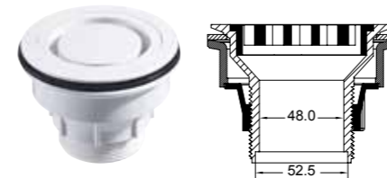
COD.181662 Shower Base Waste 2" White Bermuda 108x80x2"
